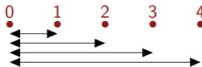
Figure 6. Regular spacing between n points
