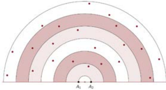
Figure 16. Half-crowns modulo 3
