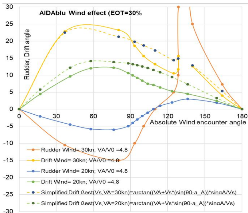
Figure 5. Rudder and drift angle versus absolute wind encounter angle for wind speeds of 20kn and 30kn (equilibrium on straight track, EOT=30%, i.e. constant ship speed V_0=6.2 kn)
