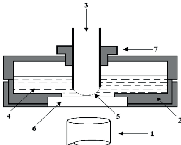
Fig. 1. Cell for investigation of microscopic wetting thin liquid films. 1 - microscope, 2 - teflon vessel, 3 - vertical capillary tube, 4 - liquid phase (aqueous solution), 5 - hemispherical meniscus, 6 - solid substrate ( \text{SiO}_2 -glass plate), 7 - teflon ring
