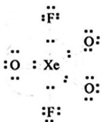
Fig. 2. Lewis structure of \text{XeO}_3\text{F}_2
