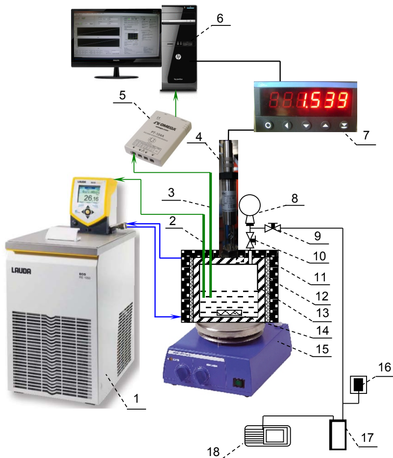
Figure 2. The experimental installation for the vapor pressures at T=(333.15 to 468.15) K: (1) Thermostat Lauda Gold RE-415 G; (2) platinum resistance thermometers PT-100 for the control of the measuring cell temperature by the thermostat; (3) platinum resistance thermometer PT-100 for the control of temperature of the measuring cell; (4) Pressure transmitter 35 X HTC Omega GmbH and Co.; (5) Omega PT-104A Channel RTD Input Data Acquisition Module for the measuring of temperature; (6) PC; (7) Manual pressure signal conditioner; (8) Flask for the sample; (9), (10) valves; (11) insulation of measuring cell; (12) heat transfer reservoir; (13) measuring cell; (14) magnet; (15) magnetic stirrer; (16) vacuum indicator; (17) liquid nitrogen trap with cold finger; (18) vacuum pump.
