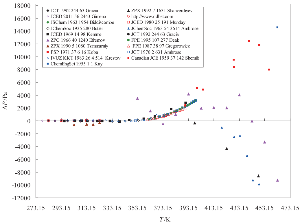
Figure 4. Plot of absolute deviation of experimental P_{exp} . and literature P_{lit} . vapor pressure values of 1-butanol versus temperatures T/K .
