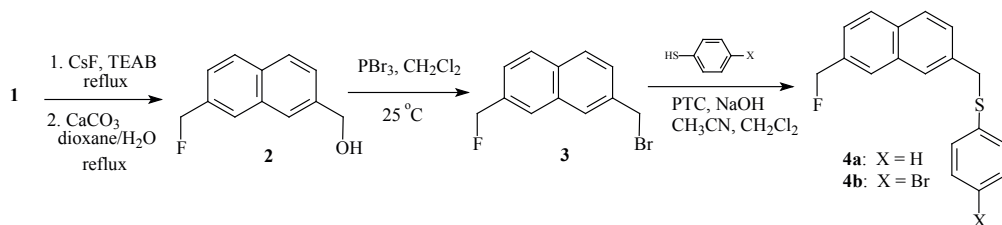
Fig. 2. Multistep synthesis of 2-fluoromethyl-7-(phenylsulfanylmethyl)naphthalene ( 4a ) and 2-fluoromethyl-[(4-bromophenyl)sulfanylmethyl]naphthalene ( 4b )
