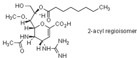
6. Laninamivir octanoate
