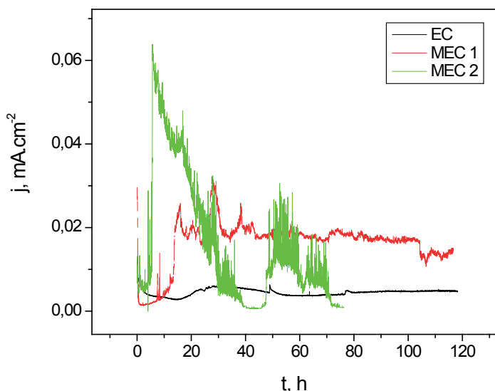
Fig. 2. Development of the current density of both MECs ( U_{\text{applied}} = 0.8 \text{ V} for MEC 1 and U_{\text{applied}} = 1.0 \text{ V} for MEC 2) and of an abiotic control (EC)
