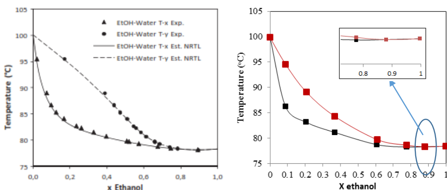
Fig. 2. Vapor-liquid equilibrium curve at 1 atm for ethanol-water mixture. (a) T-x curve; (▲) T-x Carey; (●) T-y Carey; (—) T-x NRTL; (---) T-y NRTL (Carey & Lewis, 1932); (b) T-x curve of ethanol-water experiment; (■) Dew point; (■) Boiling point (experimental data)
