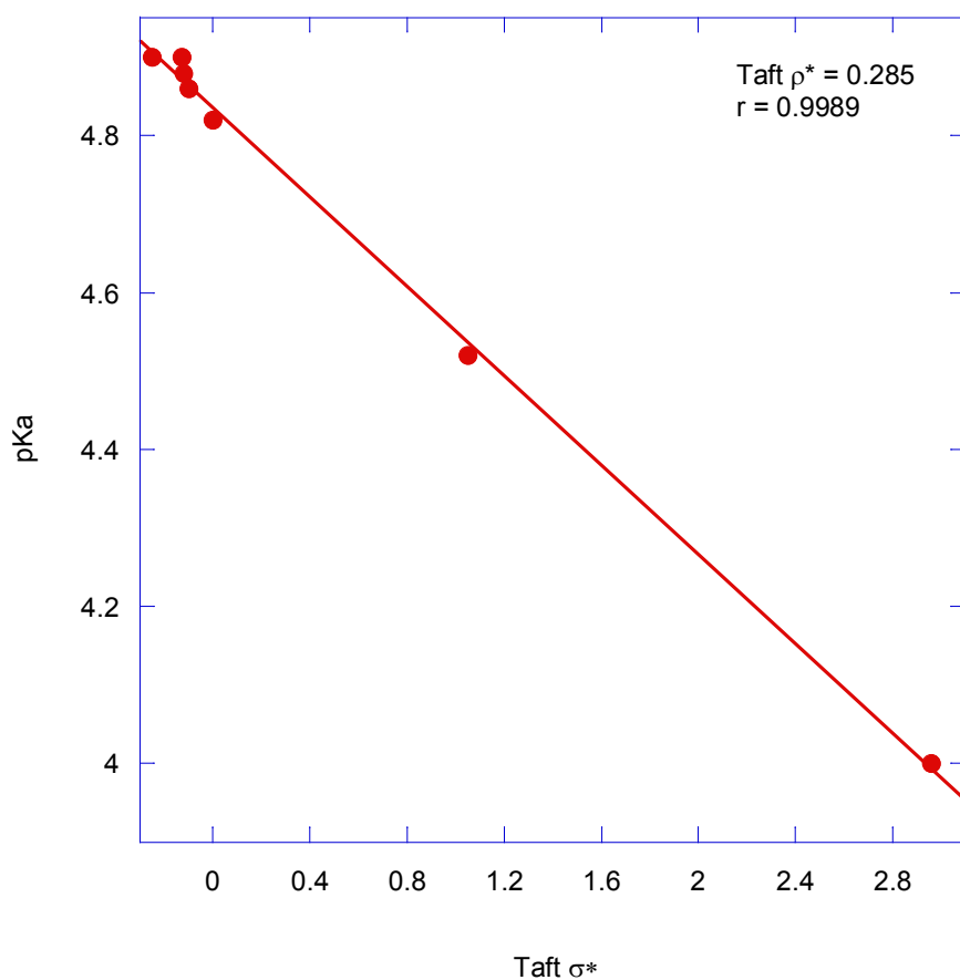
Figure 5. Plot of pK_a vs. Taft \sigma^* , i=4
